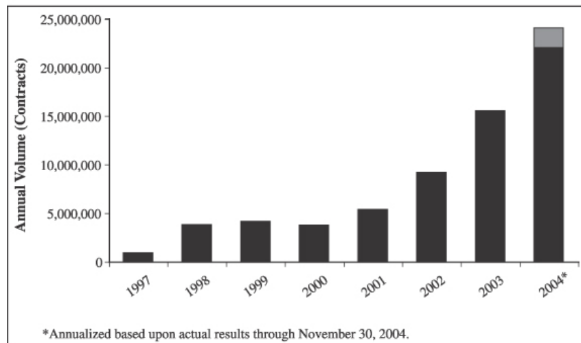
Chicago Board of Trade Annual Stock Index Futures and Options Volume 1997 through November 2004
